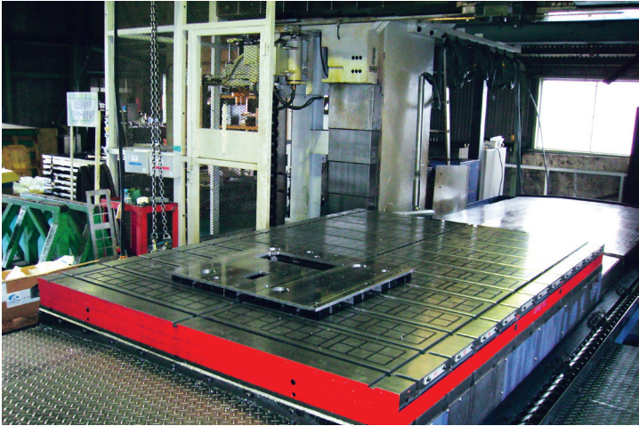
Permanent electromagnetic chuck for cutting (An example of large size)
